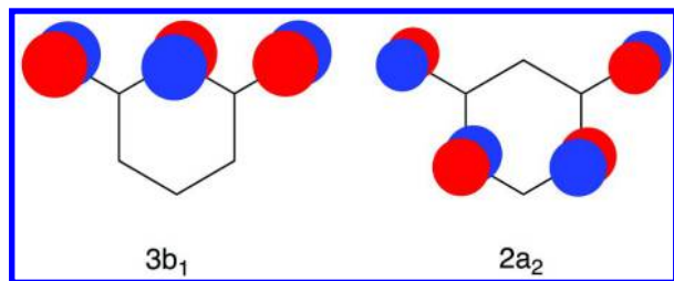
Figure 17. Schematic depiction of the Hückel NBMOs of MBQDM .
