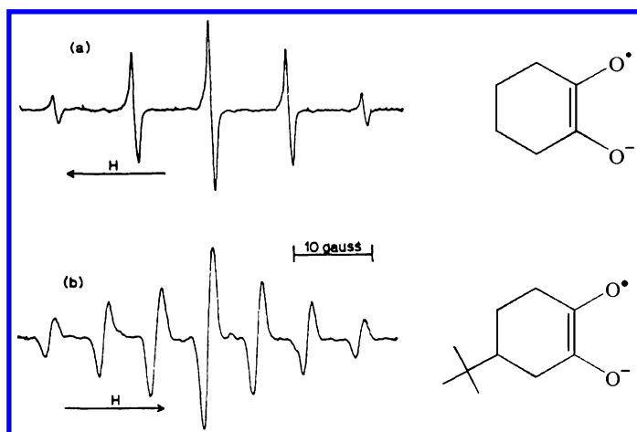
Figure 19. ESR spectra of (a) 1,2-cyclohexanesemidione and (b) 4-t-butyl-1,2-cyclohexanesemidione.
