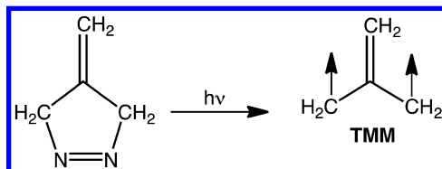
Figure 4. The generation of triplet TMM by photolysis of 4-methylenepyrazoline (27).
