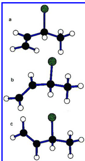
Figure 1. 3-Chloro-1-butene conformers
